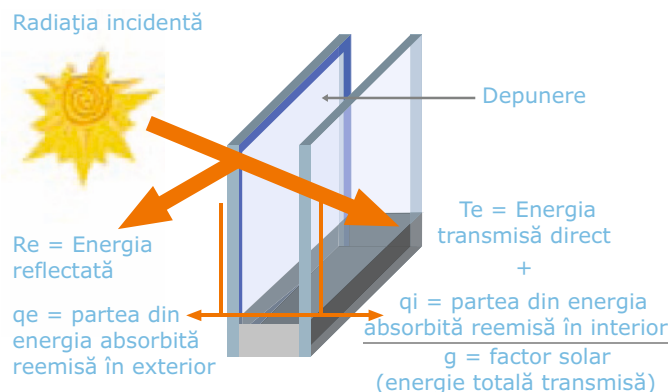
Transmisia energetică Te SGG COOL-LITE® ST
